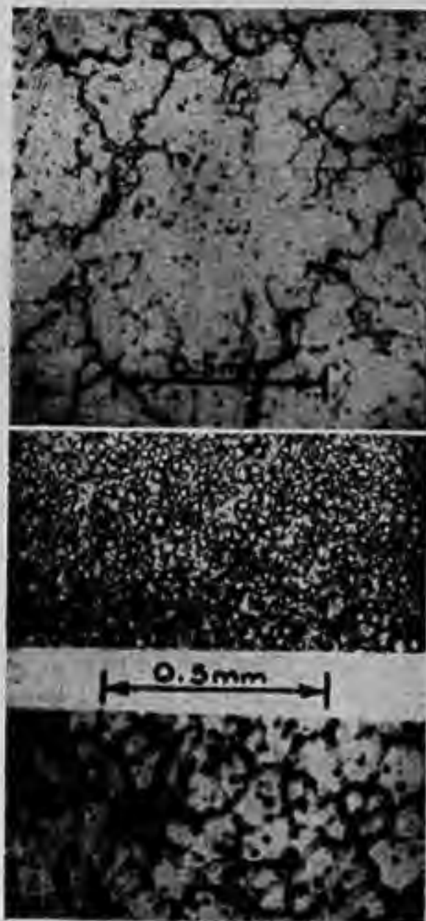
Fig. 10.—Comparison of the structure of AS superheated with die-cast Elektron Z5Z.
